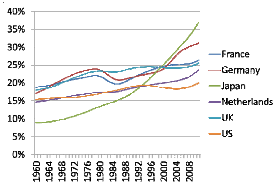
Figure 10 – Dependency ratios
